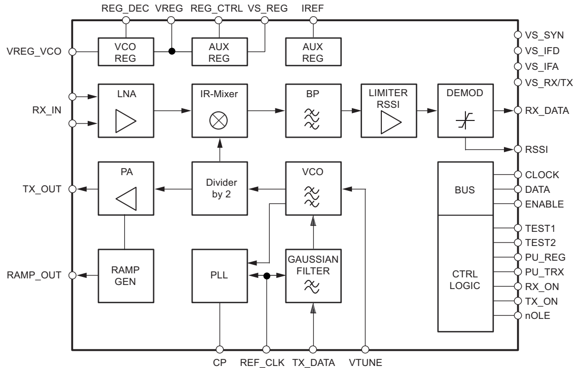
Figure 1-1. Block Diagram
